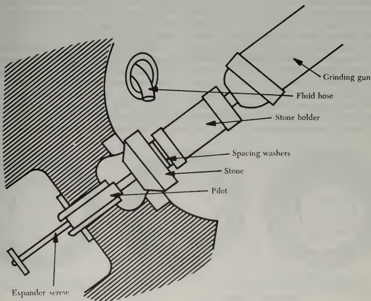
FIGURE 10-8. Valve seat grinding equipment.
